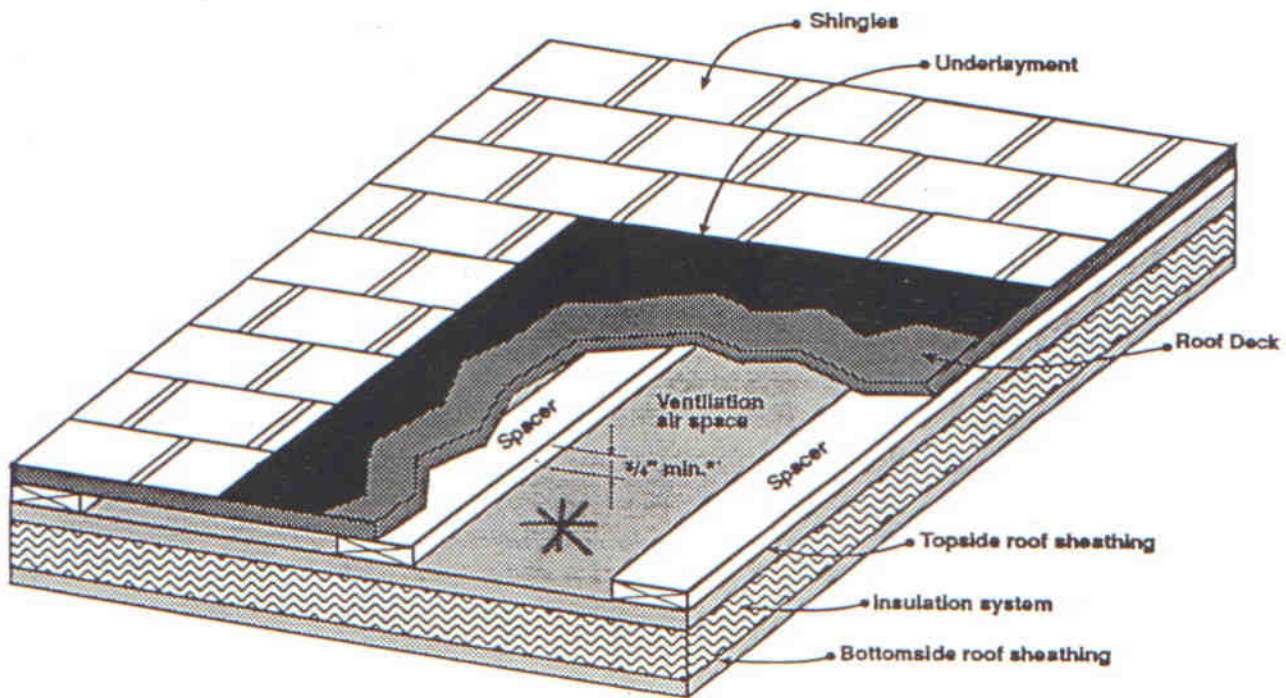
Figure B: Complete roofing assembly including spacers for ventilation
